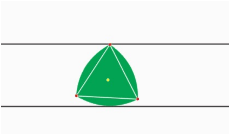
Figure 2: One of the infinitely many non-circular shapes with constant width.
